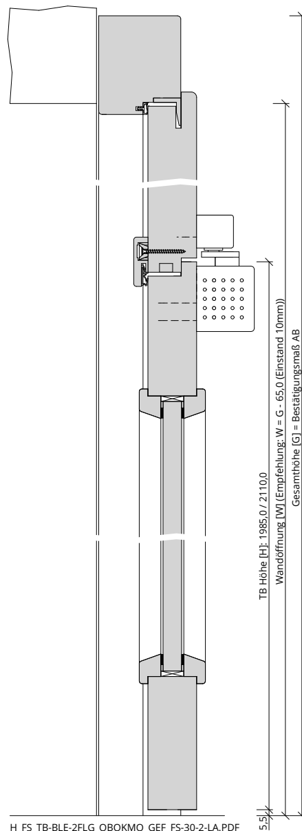
H_FS_TB-BLE-2FLG_OBOKMQ_GEF_FS-30-2-LA.PDF
