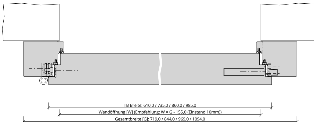
Q_FS_TB-BLE-1FLG_SH_GEF_FS-30-1-DF-SK3-RD.pdf
