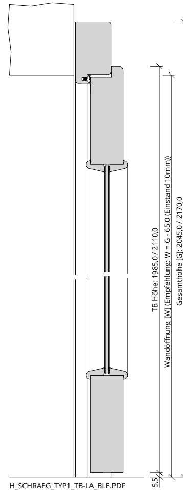
H_SCHRAEG_TYP1_TB-LA_BLE.PDF
