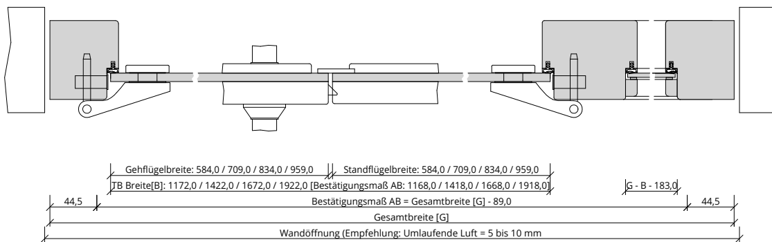
Q_DT-WF_WF1_GG_BLO_2FLG.pdf
