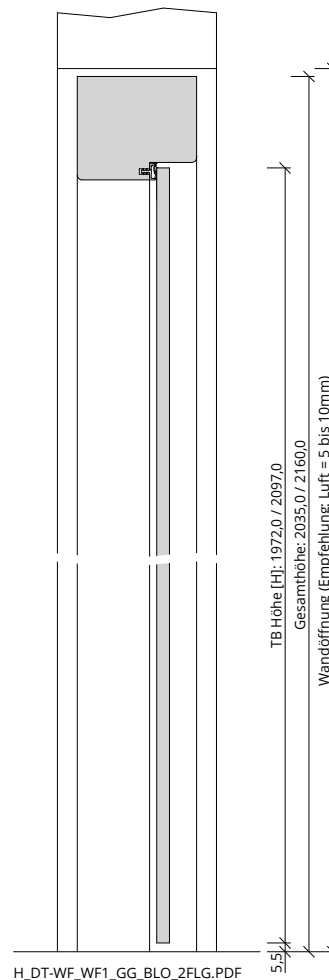
H_DT-WF_WF1_GG_BLO_2FLG.PDF
