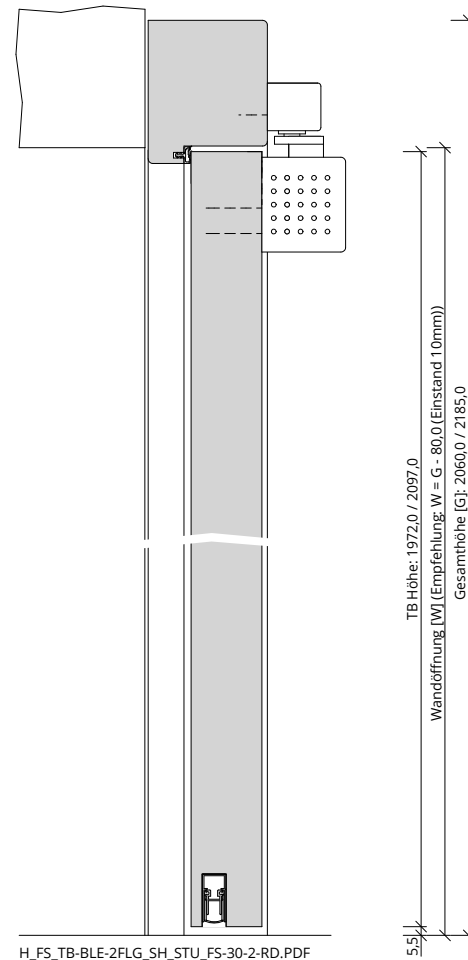
H_FS_TB-BLE-2FLG_SH_STU_FS-30-2-RD.PDF
