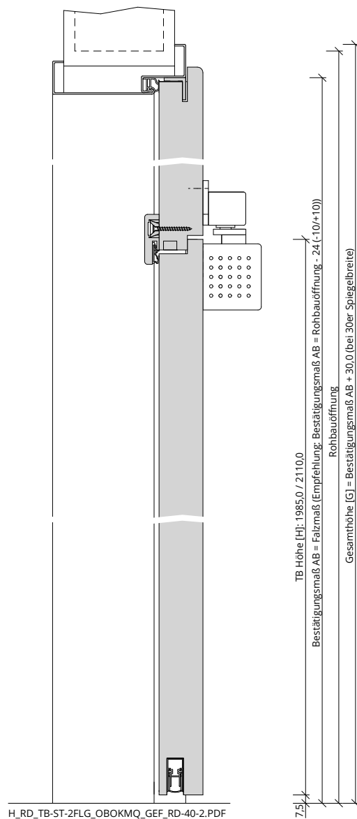
H_RD_TB-ST-2FLG_OBOKMQ_GEF_RD-40-2.PDF
