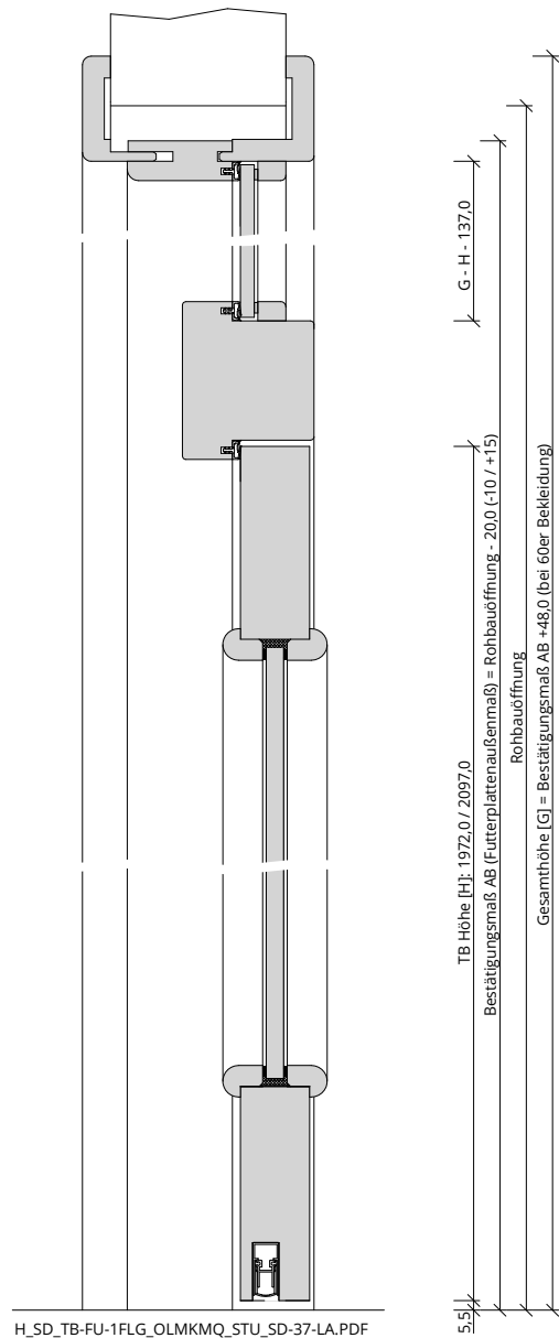
H_SD_TB-FU-1FLG_OLMKMQ_STU_SD-37-LA.PDF
