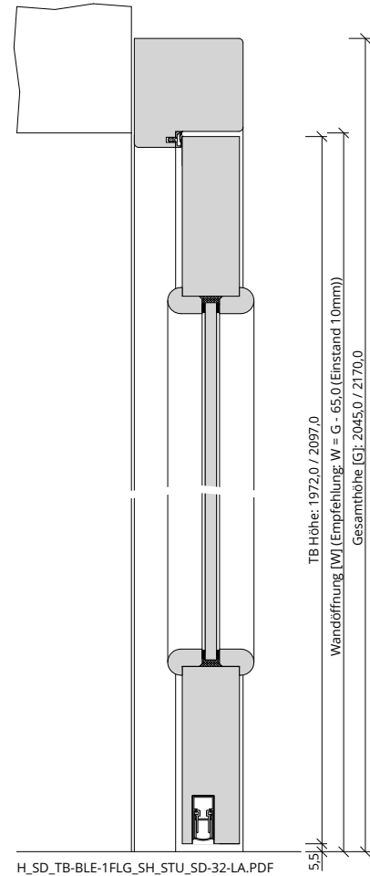
H_SD_TB-BLE-1FLG_SH_STU_SD-32-LA.PDF
