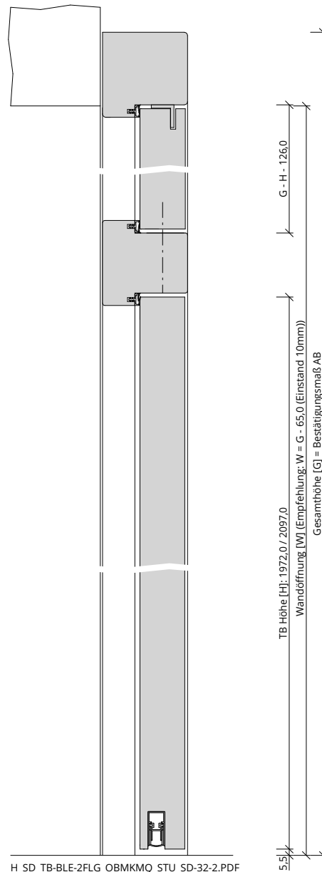
H_SD_TB-BLE-2FLG_OBMKMQ_STU_SD-32-2.PDF
