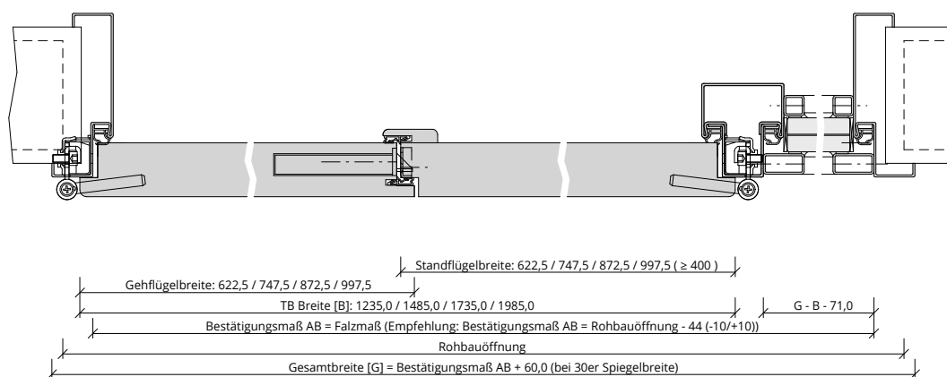
Q_SD_TB-ST-2FLG_WF1_GEF_HSD-43-2.PDF
