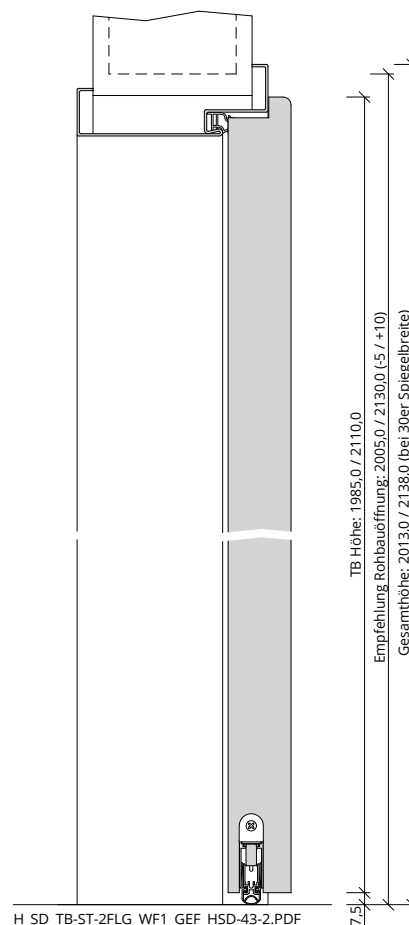
H_SD_TB-ST-2FLG_WF1_GEF_HSD-43-2.PDF
